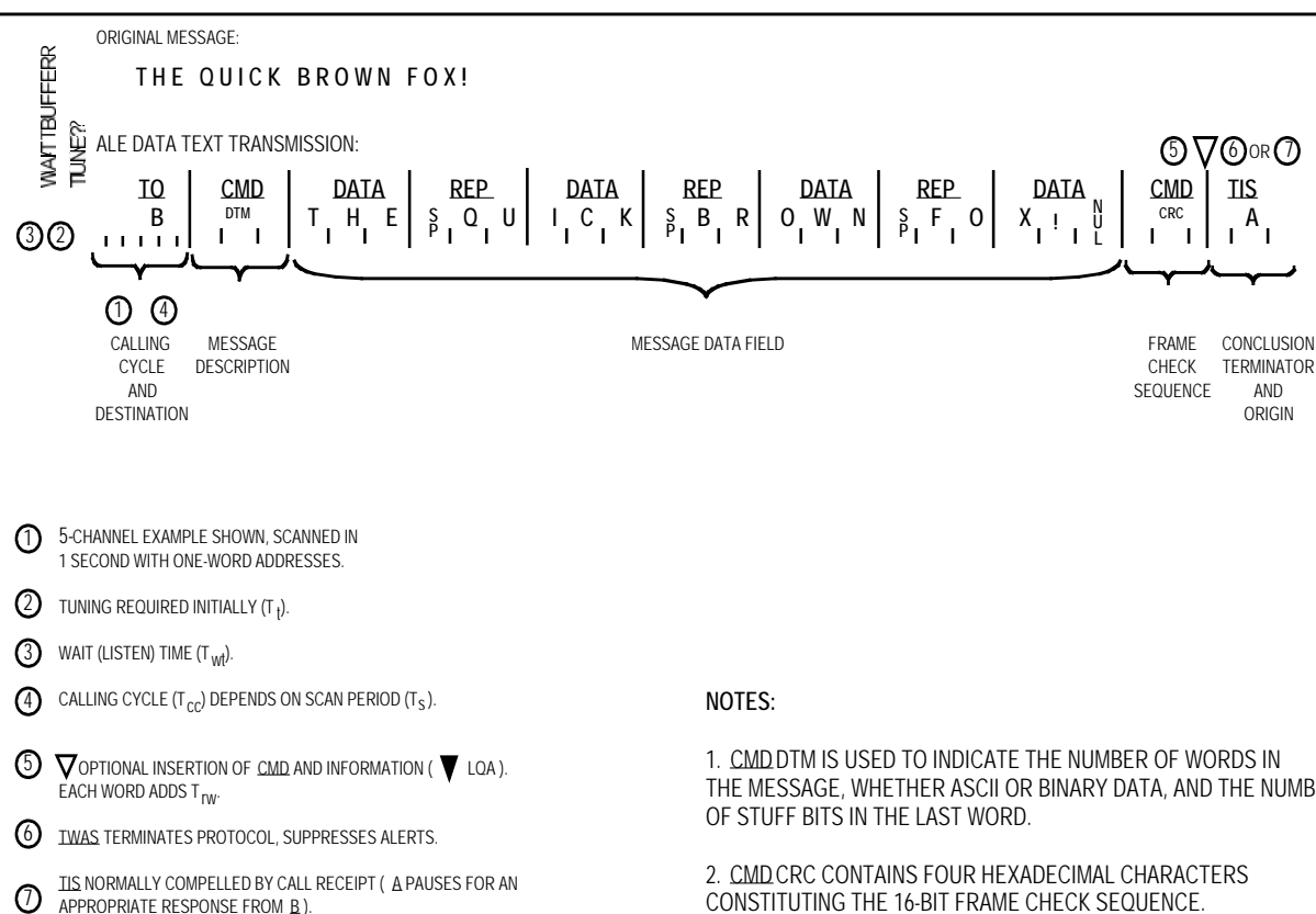
FIGURE A-47. DTM structure example.
