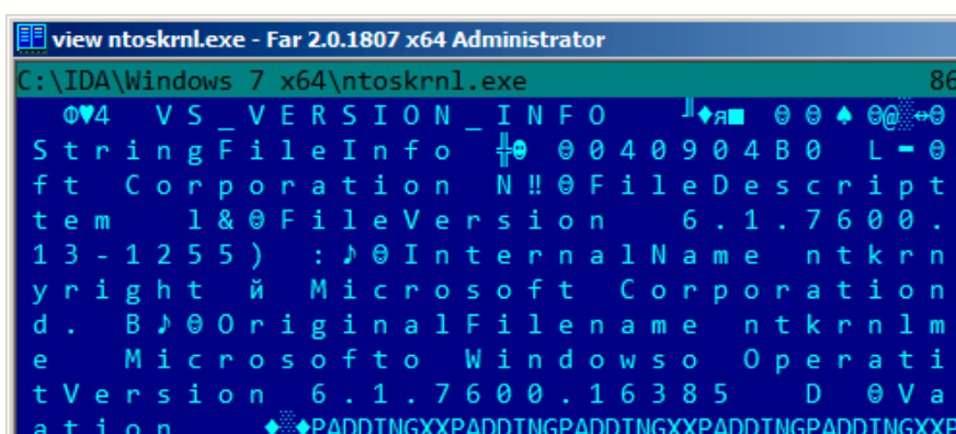
Figure 39.4: Hiew
