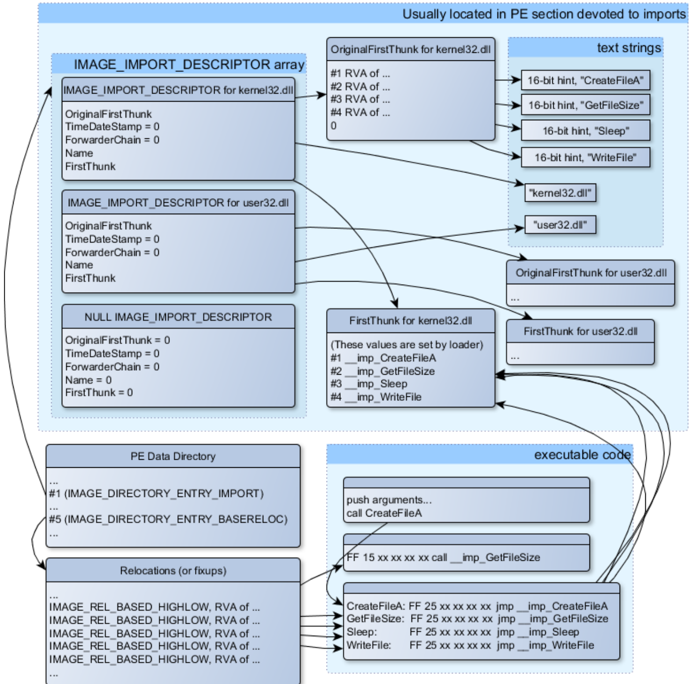
Figure 50.1: The scheme, uniting all PE-file structures related to imports
