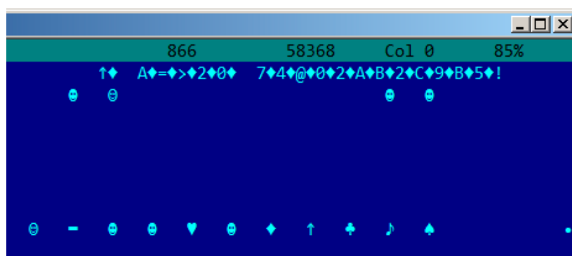
Figure 39.5: Hiew: UTF-16LE
