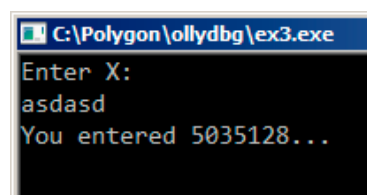
Figure 6.9: console window
