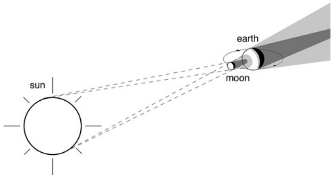
Fig. 13.2 Solar eclipse
