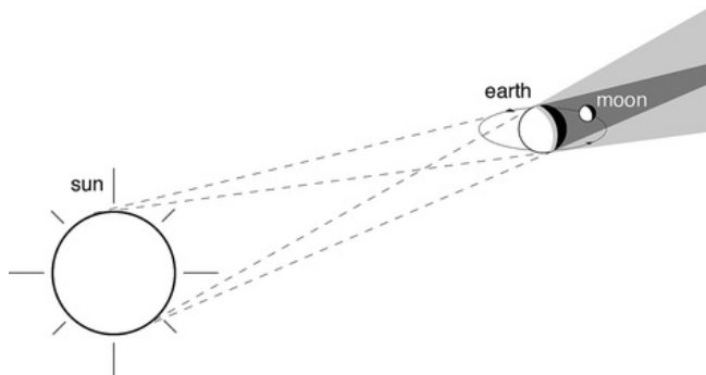
Fig. 13.4 Lunar eclipse
