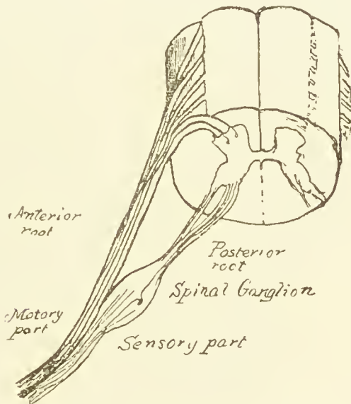
SPINAL CORD.
