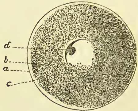
A CELL.
