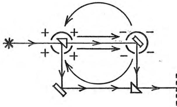
Krafft's Interferometer
