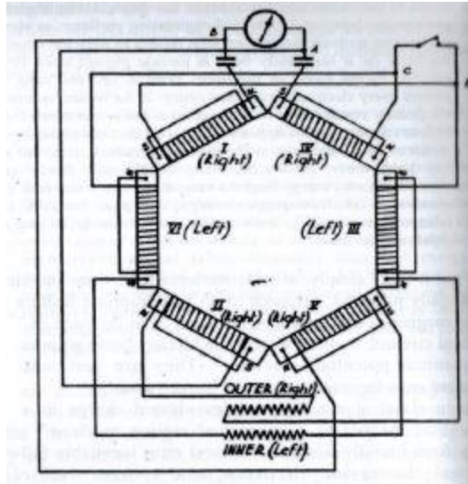
Schematic of the Kohler Coil
