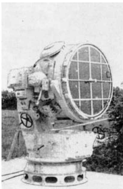
German Infrared Equipment For Naval Vessels
