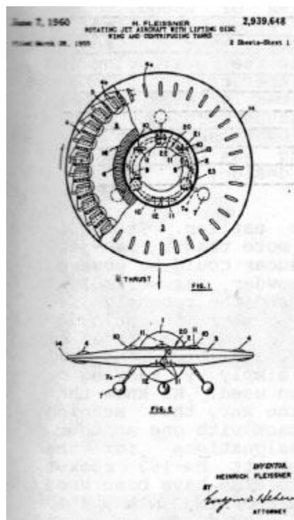
Fleissner U.S. Patent # 2,939,648, "Rotating Jet Aircraft with Lifting Disc Wing and Centrifuging Tanks ", Overhead and Frontal Views
