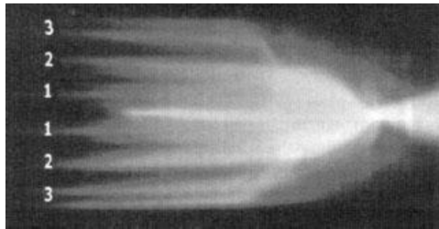
Laboratory-Produced Plasma Pinch “Flower”
