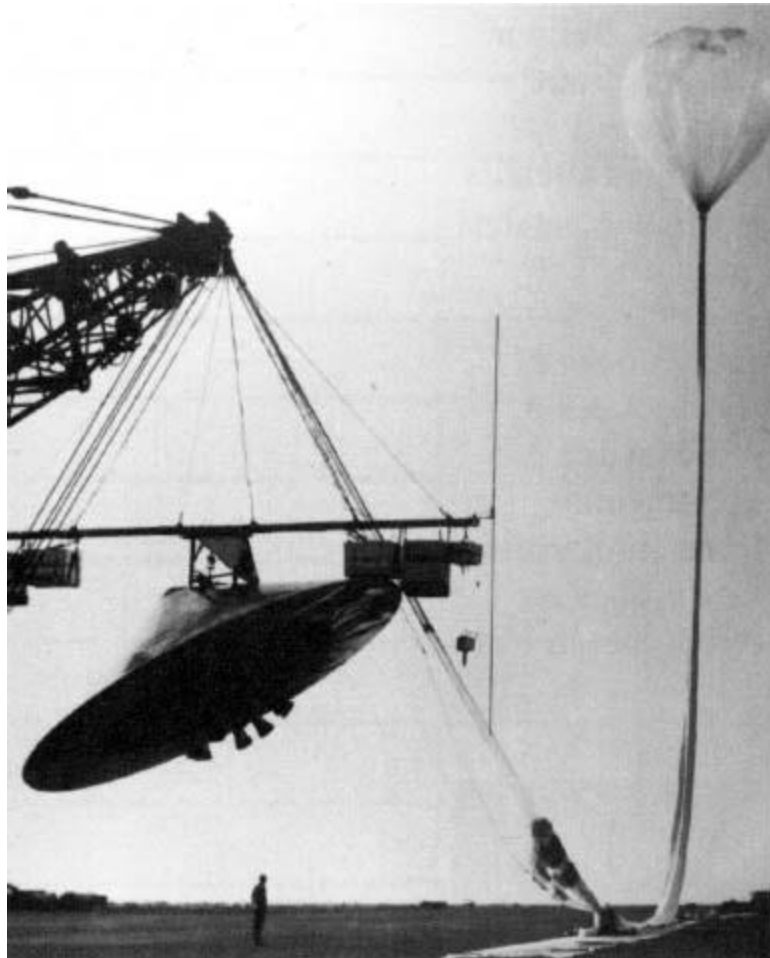
High Altitude Balloon Launching of Voyager Spacecraft 3
