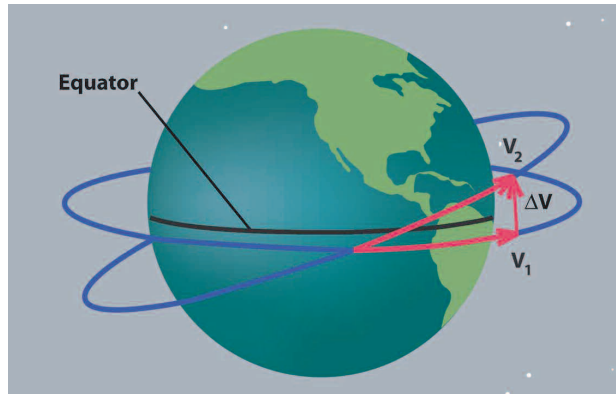
Figure 6.4. This figure shows two orbits with different inclinations. The velocity vector for a satellite in each orbit is denoted by the arrows labeled V_1 and V_2 . For the satellite to change its orbit from one plane to the other, the satellite's thrusters must produce a \Delta V large enough to rotate its velocity from V_1 to V_2 .
