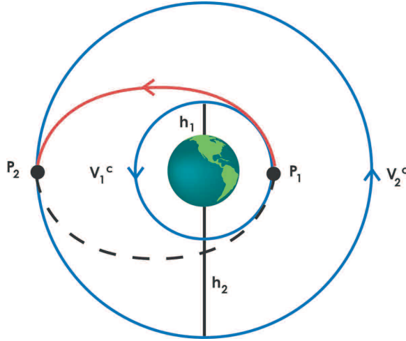
Figure 6.2. This figure shows the elliptical Hohmann transfer orbit between two circular orbits, the initial one with altitude h_1 and the final one with altitude h_2 . \Delta V_1 is applied at point P_1 and \Delta V_2 at P_2 . The satellite travels only half an orbit on the transfer orbit; it does not travel the half of the ellipse indicated by the dashed line.
